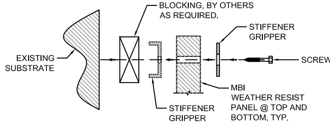
B L-11 HARDWARE ATTACHMENT DETAIL SCALE: NA
