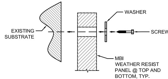
D L-11 ALTERNATE - HARDWARE ATTACHMENT DETAIL SCALE: NA
