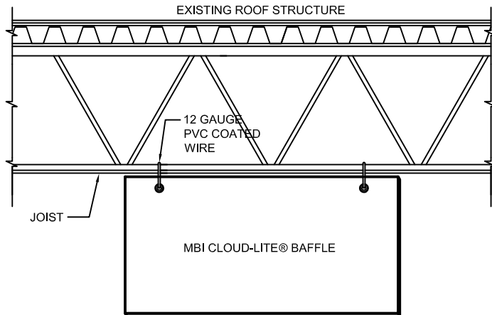
3 CL-03A FRONT ELEVATION SCALE: NA
