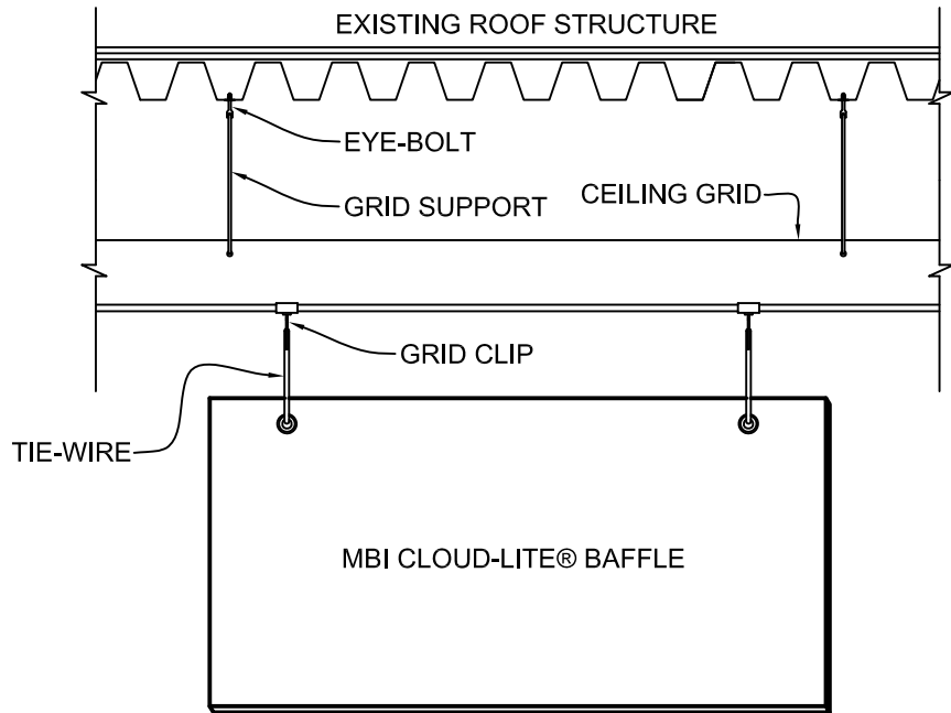
3 CL-04 FRONT ELEVATION SCALE: NA
