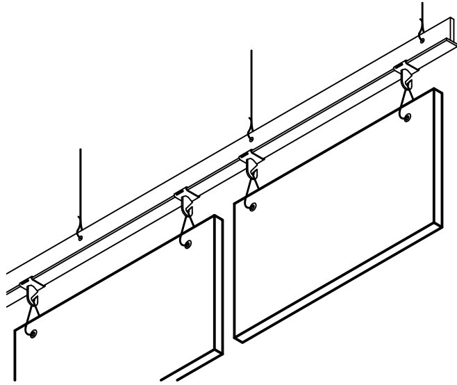
1 CL-04 VIEW FROM BELOW SCALE: NA
